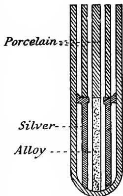
FIG. 81.—Sahmen and Tammann's dilatometer.
